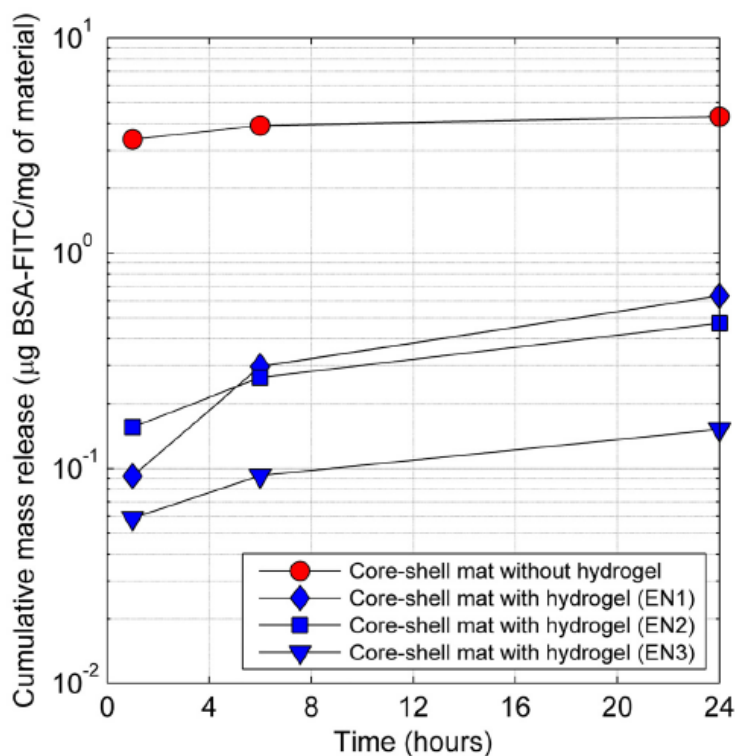
Fig. 5.2. Cumulative release of BSA-FITC from: core-shell mat with NIPA hydrogel in the core (EN1-EN3), and core-shell mat with protein water solution in the core (without hydrogel). For a better visibility of results, the y-axis is in a logarithmic scale. Standard deviation was less than 5%.
