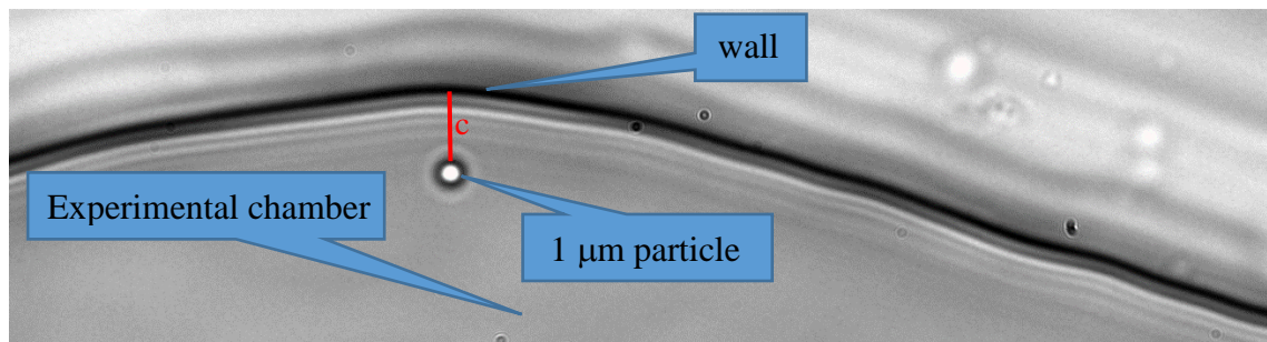
Fig. 3.3. Starting position of 1\ \mu\text{m} particle trapped by OT during a single experiment inside the chamber. The red line indicates the direction of the particle motion tagged by OT into the wall; c is the shortest distance from the wall. The black contour in the image indicates the wall.
