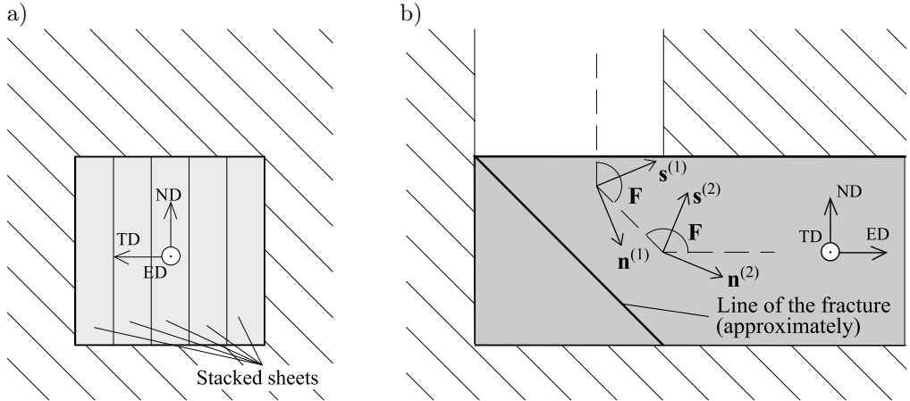
FIG. 2. The schematic showing: a) the stacking of sheets in the channel, b) the fracture of the material. The figure also shows the vectors describing the direction and plane of shearing in two simple shear used for modeling the material's deformation.
