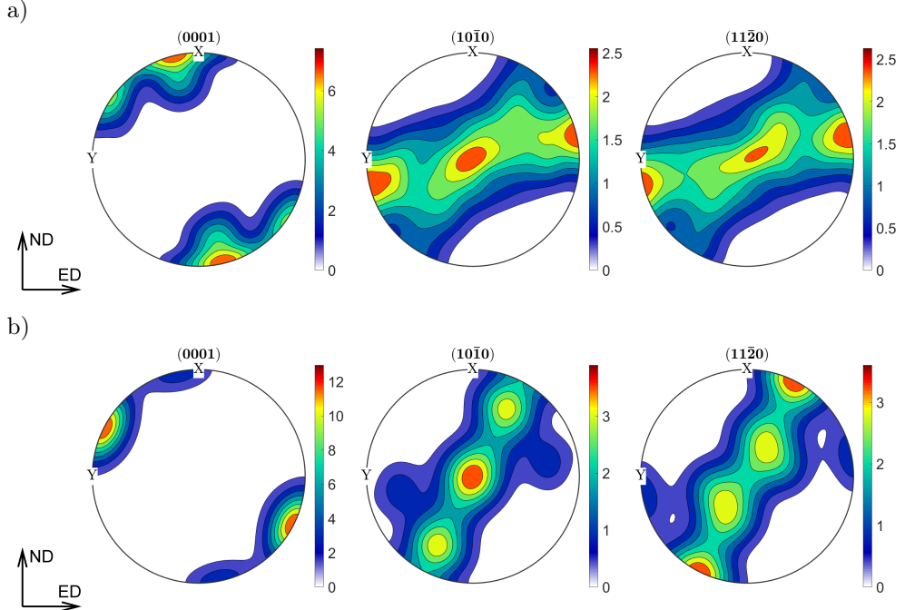
FIG. 4. \{0001\} , \{10\bar{1}0\} and \{11\bar{2}0\} pole figures plotted for the texture: a) initially supplied in the simulation, b) after one ECAP pass. The texture has been plotted using the MTEX software [47].
