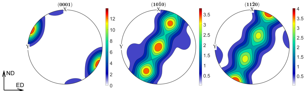
FIG. 9. \{0001\} , \{10\bar{1}0\} and \{11\bar{2}0\} pole figures plotted for the texture after one ECAP pass simulated using the parameters established for AZ31B rod (Table 2). The texture has been plotted using the MTEX software [47].
