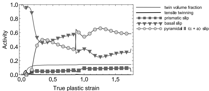
FIG. 7. Slip and twinning system activities in the simulation of one ECAP pass simulated using the initial random texture.
