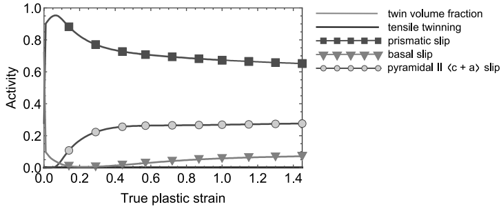
FIG. 6. Slip and twinning system activities in the simulation of rotary swaging.
