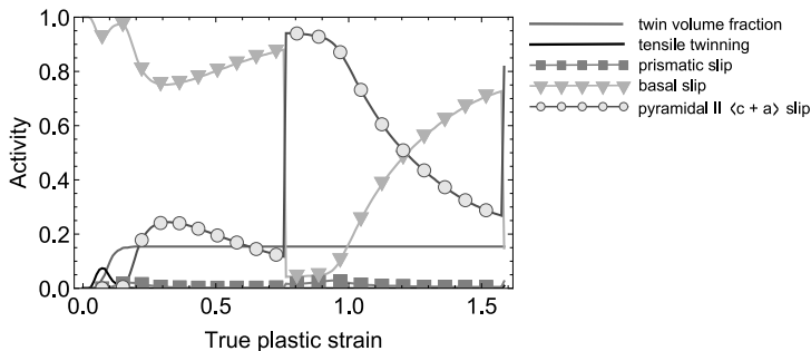
FIG. 3. Slip and twinning system activities in the simulation of one ECAP pass.
