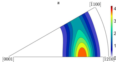
FIG. 10. Inverse pole figures of the wire axis direction obtained in the simulation of rotary swaging after applied strain \eta = 1.45 using the parameters established for AZ31B sheet (Table 1). The texture has been plotted using the MTEX software [47].
