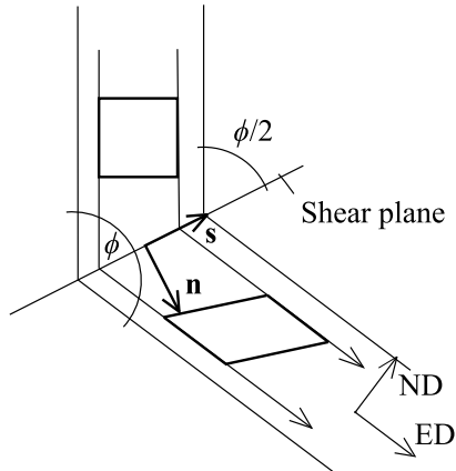
FIG. 1. Schematic showing the simple shear as applied in ECAP [10].
