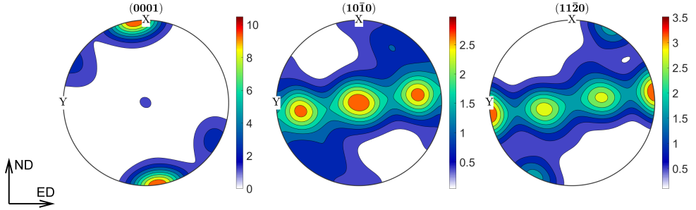
FIG. 8. \{0001\} , \{10\bar{1}0\} and \{11\bar{2}0\} pole figures plotted for the texture after one ECAP pass simulated using the initial random texture. The texture has been plotted using the MTEX software [47].
