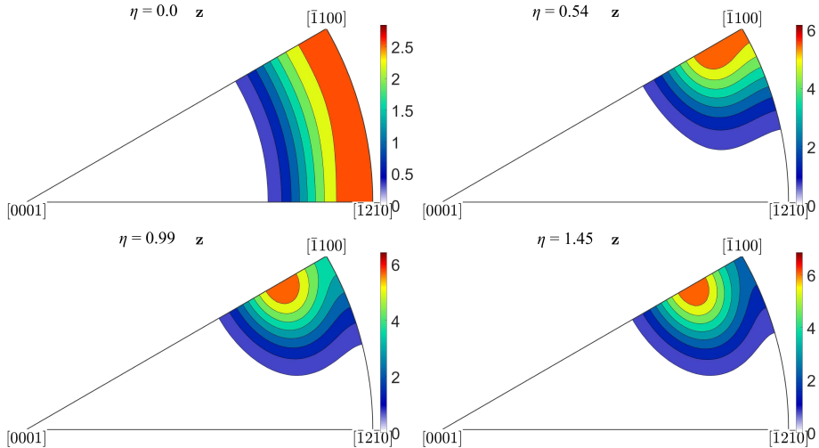
FIG. 5. Inverse pole figures of the wire axis direction obtained in the simulation of rotary swaging after various amounts of strain ( \eta = 0 means the initially supplied texture). The texture has been plotted using the MTEX software [47].
