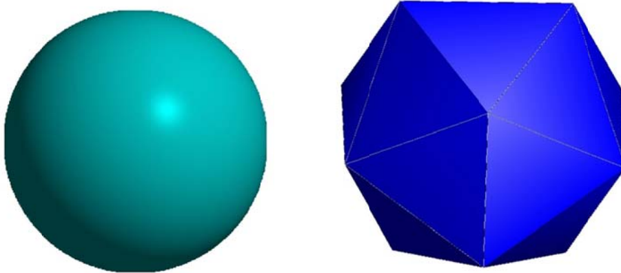
Fig. 8. Conversion of a sphere surrounding a point into an icosahedron for contact detection
