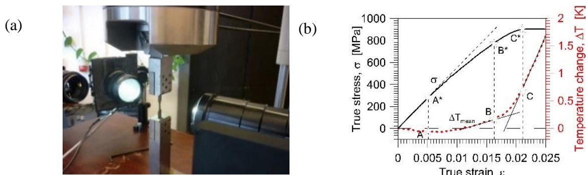
Figure 1. a) Experimental set-up used for investigation of deformation and thermal fields. b) Stress \sigma and the mean temperature change ( \Delta T_{\text{mean}} ) vs. mean strain \epsilon at strain rate of 10^{-2}\text{s}^{-1} up to \epsilon = 0.025 .
