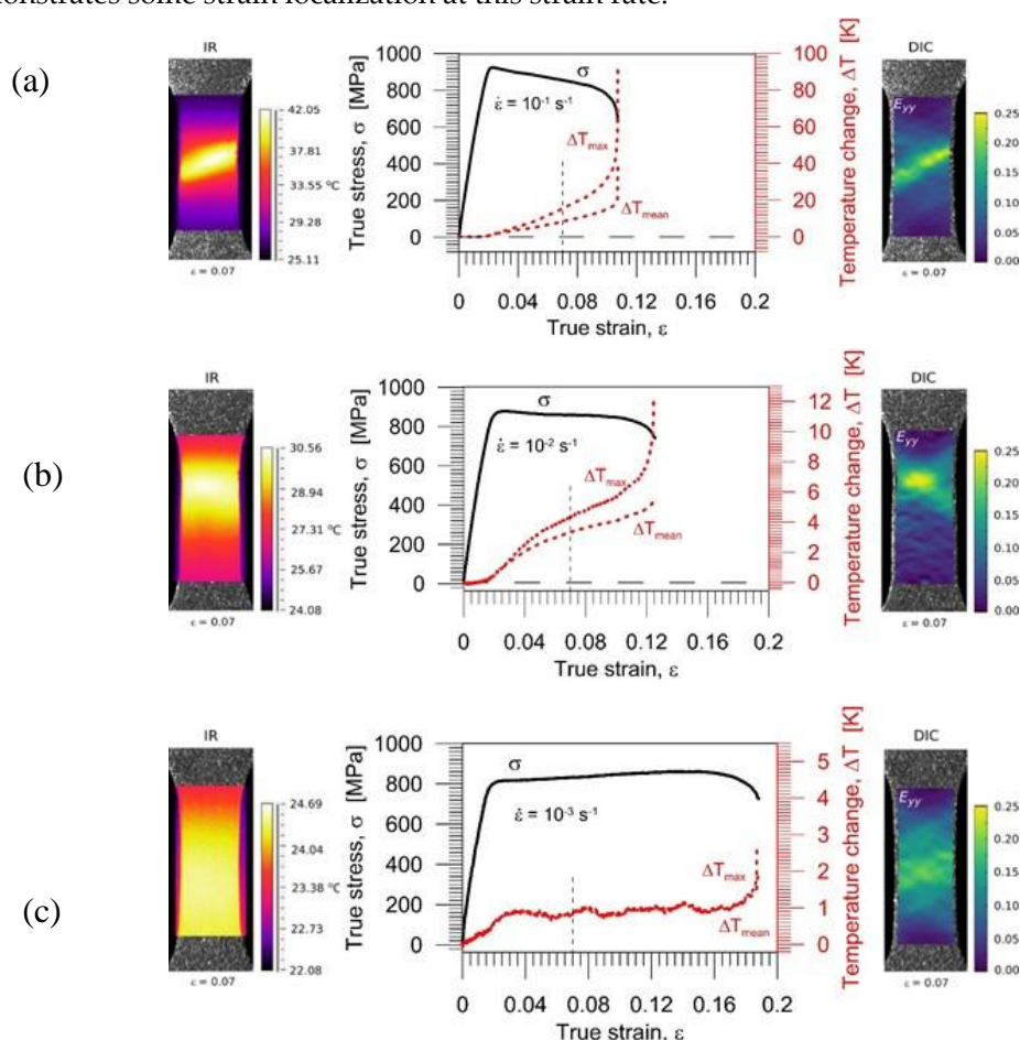
Figure 2. Stress \sigma , \Delta T_{\text{max}} and \Delta T_{\text{mean}} temperatures vs. strain \epsilon for strain rates: (a) 10^{-1} \text{ s}^{-1} , (b) 10^{-2} \text{ s}^{-1} , (c) 10^{-3} \text{ s}^{-1} . In addition, thermograms (left) and corresponding \epsilon_{yy} strain component distribution (right).
