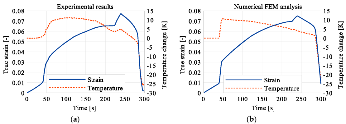
Figure 10. Strain and temperature variations vs. time for the loading program (2): 3-min loading interruption in the middle of the LMT: (a) experimental data; (b) numerical results.
