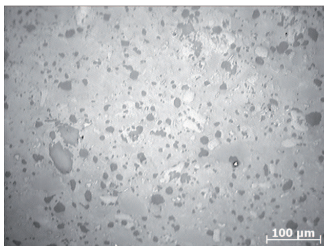
Fig. 5. Image of the structure at the boundary part of the sample stressed up to 460 MPa, magnification 200x. Dark areas remaining after crushed out particles of cullet and quartz grains of different size constitute about 7.5% of surface. Almost all bigger quartz grains contain internal cracks. Damage of mullite and corundum phases are only incidental
