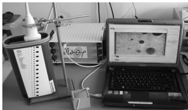
Fig.2. Experimental set-up for RF data acquisition
