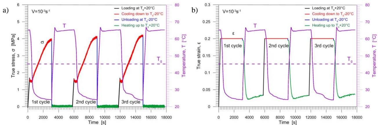
Fig. 1. Results obtained during the SMP three thermomechanical loading: a) true stress \sigma and temperature T vs. time; b) true strain \epsilon and temperature T vs. time
