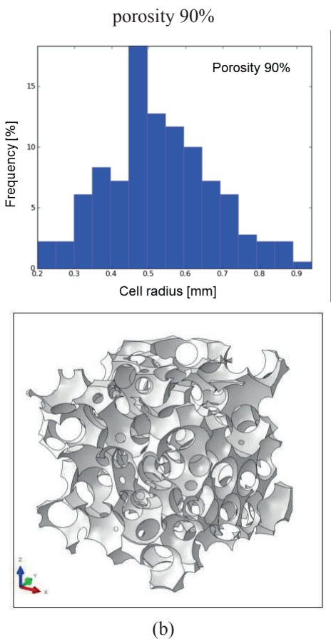
Fig. 7. The generated foam structures, (a) porosity 86% and (b) porosity 90%, histogram of cell size distribution (top) and general view of the foam structure (bottom)
