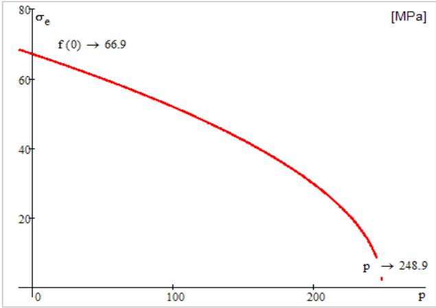
Fig. 3. The arm of the paraboloid being the representation of the Burzyński yield criterion for the polycarbonate in the surface (\sigma_e, p) .
