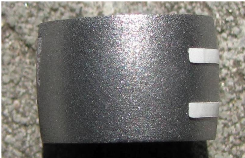
Fig. 6. Picture of the deformed cylindrical specimen.
