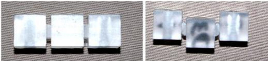
Fig.1. The sample 12x12x40 [mm] with the shearing zone 6x6x2 [mm] prepared for a double shear test before and after deformation.
