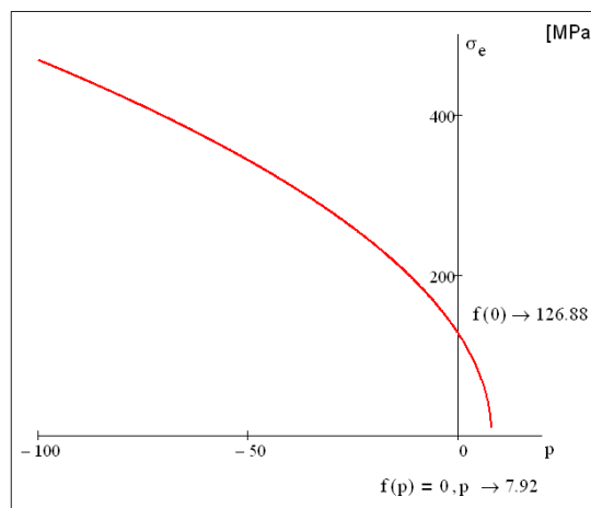
Fig.10. A half parabola being the representation of the Burzyński failure criterion for the MMC composite 75%Cr - 25% Al 2 O 3 (M).in the coordinates (\sigma_e, p) .
