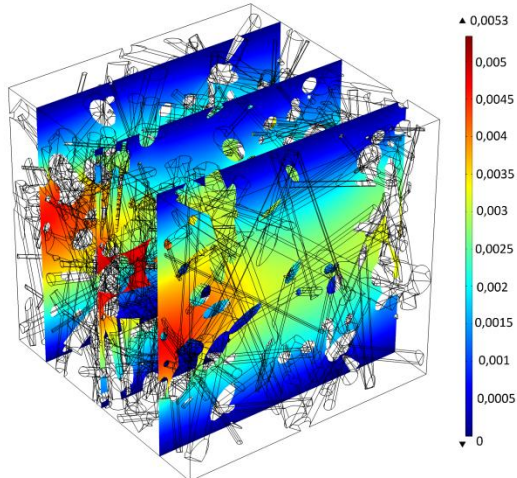
Figure 9. Simulated drug concentration distribution in fluid between randomly oriented fibers after 14 days of release r = 2.0\mu\text{m} , \mathbf{K}_t = [0.36 \ 0.33 \ 0.31] .
