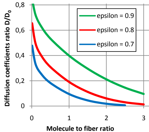
Figure 4. Variation of the relative diffusion coefficients for three different porosities of the material in the function of drug molecule to fiber ratio.
