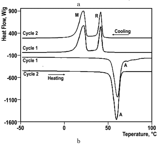
Fig. 1 – DSC curves of the virgin NiTi alloy (a) and DSC curves of ion-implanted alloys indicating a two-step phase transformation occurred during cooling (b)
