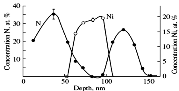
Fig. 6 – Depth profiles of the element concentrations obtained from energy spectra of the NiTi sample surface after double implantation of N ions at a dose of 10^{18} \text{ cm}^{-2} and Ni ions at a dose of 5 \times 10^{17} \text{ cm}^{-2}
