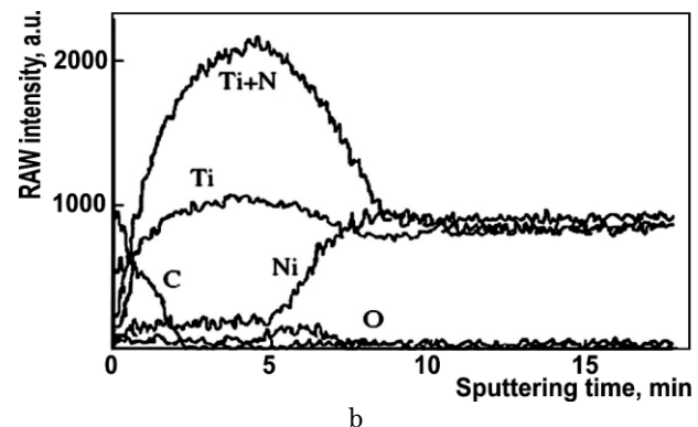
Fig. 3 – Auger electron spectroscopy data for unimplanted NiTi samples (a) and NiTi samples implanted at an energy of 65 keV and a dose of 5 \times 10^{17} ion/cm 2 (b)
