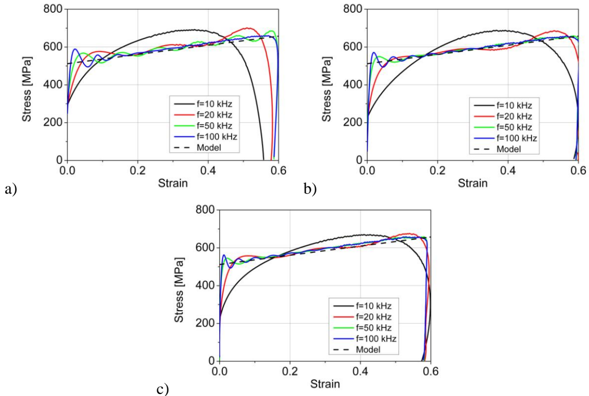
Fig. 9. Stress-Strain curves at various bridge cut-off frequencies for: a) r=\text{Inf} ; b) r=3 \text{ cm} ; c) r=1 \text{ cm}
