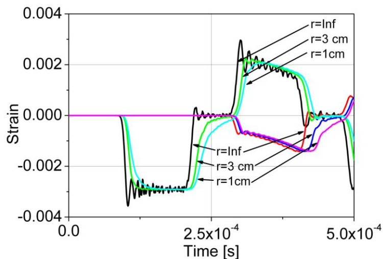
Fig. 4. Mechanical wave in bars at various striker interface radii.
