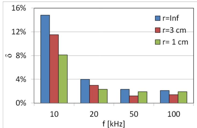
Fig. 10. Influence of striker geometry and bridge bandwidth on stress-strain error.
