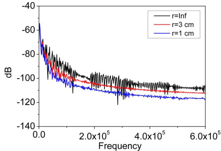
Fig. 5. Mechanical wave in bars at various striker interface radii.
