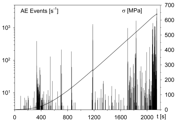
Fig. 6. Mechanoacoustic characteristic of C 130 material sample of foreign production of compressive strength 642 MPa
