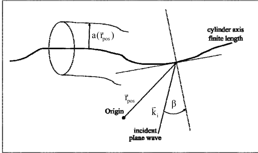
Figure 1. Scattering geometry.
