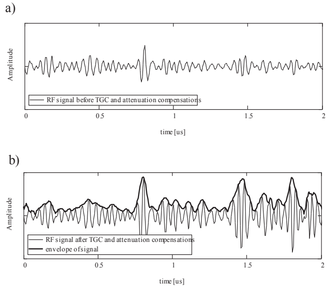
Fig. 1. RF signal before TGC and attenuation compensations (a) and RF signal after the TGC and attenuation compensations and its envelope (b)
