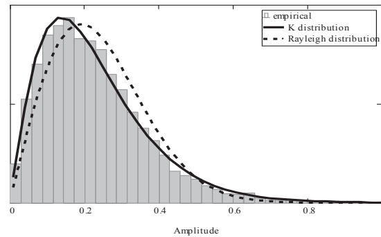
Fig. 2 Theoretical Rayleigh and K distribution and histogram of empirical data obtained at the nape of neck
