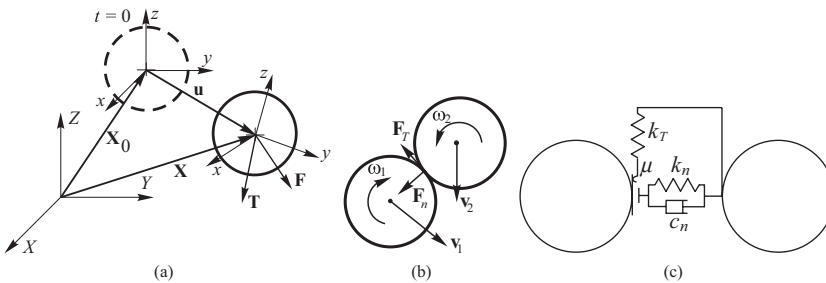
Figure 1. (a) Motion of a rigid particle. (b) Decomposition of contact force in normal and tangential components. (c) Model of the contact interface.
