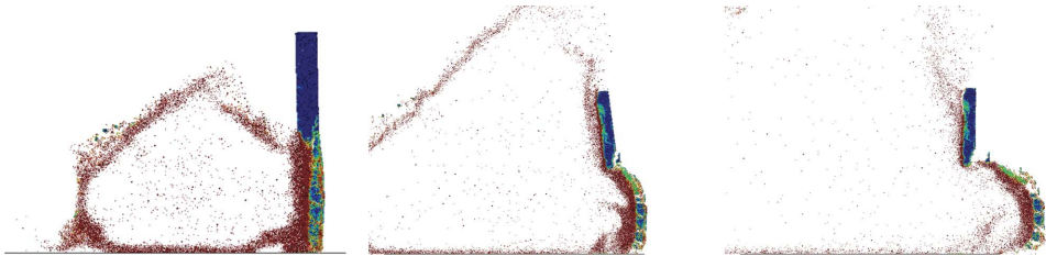
Figure 4. Masonry wall under blast load. Deformation of the wall at three time instants.
