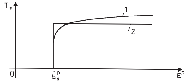
Fig. 9. Variation of the relaxation time with strain rate for mild steel (1) real case; (2) assumption for classical elasto-viscoplasticity
