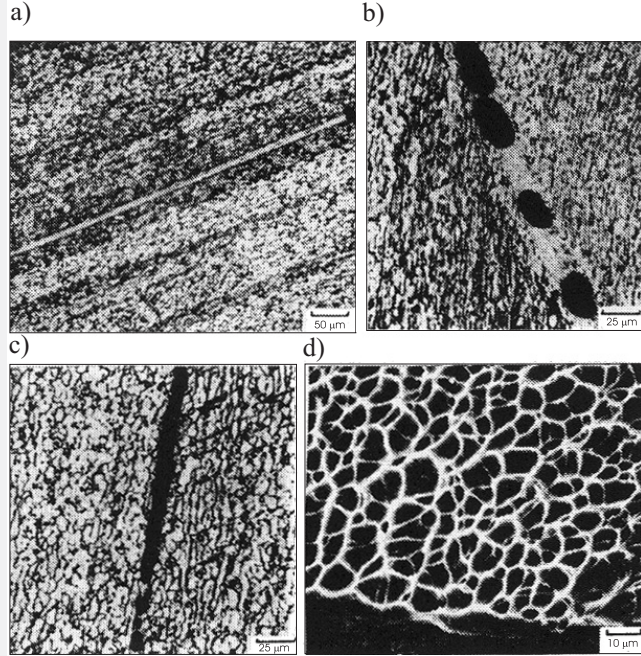
Fig. 19. Shear band in Ti6Al4V target impacted at 846 m/s (after Grebe, Pak and Meyers 1985): a) single shear band; b) microcracks in the shear band region; c) elongated macrocracks along the shear band; d) characteristic dimples observed in spall region
