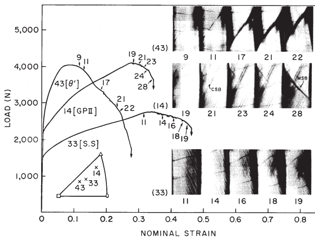
Fig. 3. Load versus engineering strain curves for various ageing treatments. Numbered photos correspond to the indicated points on the load-strain curves (after Chang and Asaro 1981)
