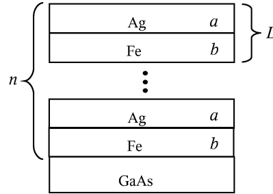
Fig. 1. Geometry of Ag/Fe nanolayer sample.
