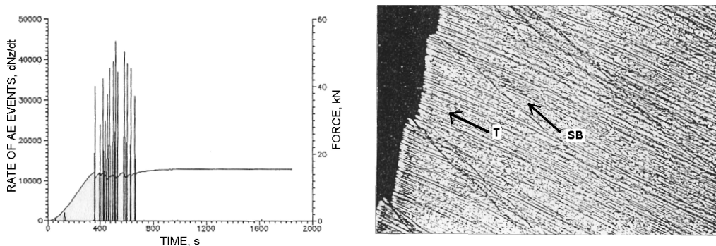
Fig. 1. The rate of AE events registered every 4 seconds, external force and corresponding microstructure (at the right: deformations twins – T and shear bands – SB ) of Ag single crystals during channel-die compression ( T = 293\text{ K} , reduction z = 31.8\% , orientation \{112\}\langle 111\rangle at image magnification \times 200 ).
