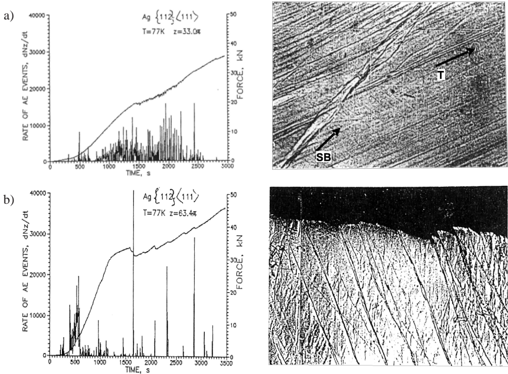
Fig. 2. AE events registered every 6 seconds, external force and microstructure of Ag single crystals of \{112\}\langle 111\rangle orientation during low temperature compression in channel-die: a) reduction z = 33.0\% , and b) reduction z = 63.4\% , at image magnification \times 200 .
