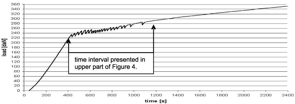
Fig. 3. External force, registered at channel-die compression of single Ag crystal with the existence of two ranges of the twinning.
