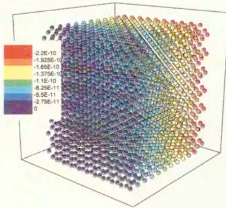
Displacements in direction Z
