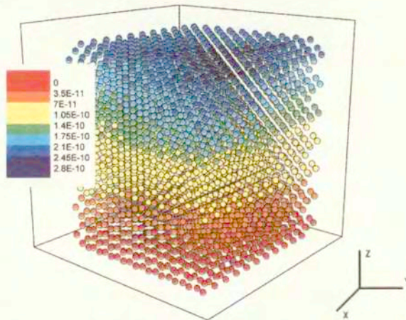
FIG. 5. Displacements resulting from the performed calculations.
