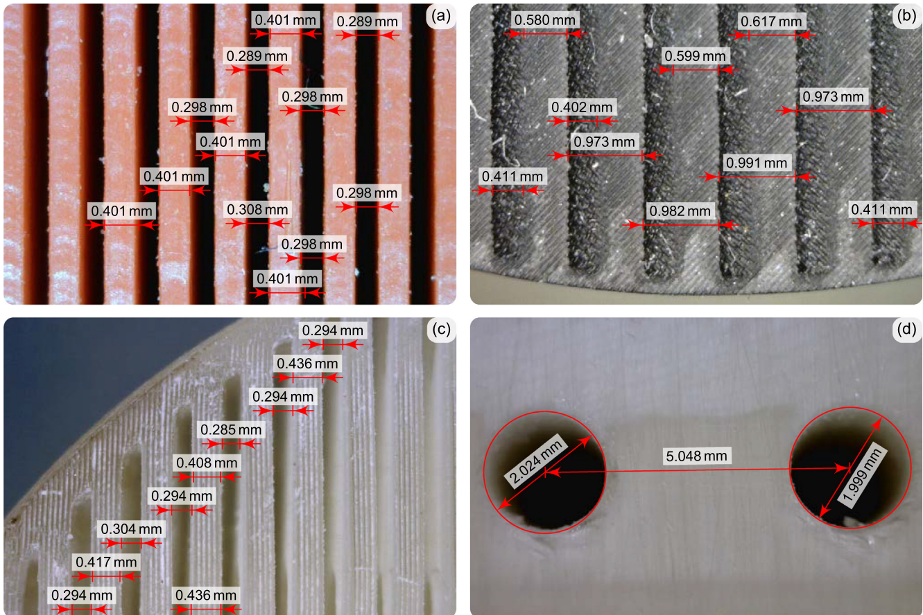
Fig. 5. Microscope measurements of the characteristic dimensions of the manufactured slitted microgeometries with: (a) \theta = 0^\circ (top view of the sample); (b) \theta = 45^\circ and the cylindrical perforation (top view of the sample); (c) \theta = 0^\circ and the cylindrical perforation (top view of the sample); and (d) \theta = 0^\circ and the cylindrical perforation (side view of the sample). The designed values are: 2w_s = 0.3 mm and 2w_w = 0.4 mm in (a, c), 2w_s/\cos \theta \approx 0.424 mm and 2w_w/\cos \theta \approx 0.566 mm in (b), and d_{\text{perf}} = 2 mm and l_{\text{perf}} \approx 4.95 mm in (d).
