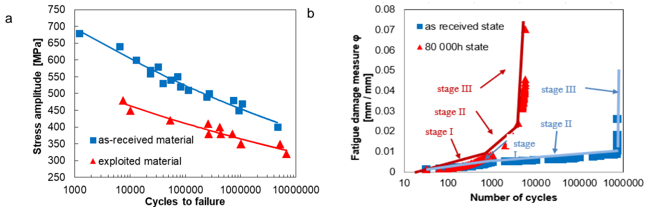
Figure 1. S-N curves for the steel in the as-received state and after exploitation (a); development of the fatigue damage for a stress amplitude of \pm 480 MPa expressed by fatigue damage measure \varphi variations as a function of number of cycles (b).
