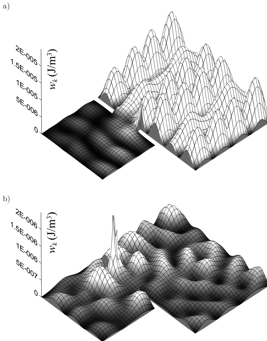
Fig. 7. Kinetic energy density w_k in the observation plane z = 1.8 m for the source positions (in meters): a) x_0 = 2.8 , y_0 = 4.2 , z_0 = 1 , b) x_0 = 7.5 , y_0 = 2 , z_0 = 1 . The source frequency is 128.6 Hz.
