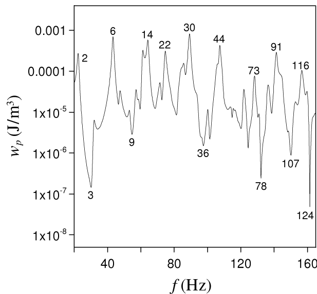
Fig. 4. Frequency dependence of the potential energy density w_p at the observation point x = 3 m, y = 5 m, z = 1.8 m for the source position x_0 = 2 m, y_0 = 3 m, z_0 = 1 m. Numbers above maxima and below minima represent the mode number n .
