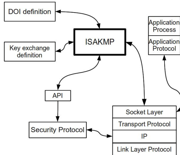
Fig. 1. ISAKMP architecture
