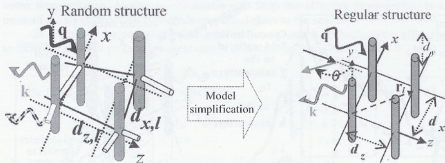
Fig. 6. Model simplification: left – full bone model (random); right – simplified model (regular), d_z = d_x = d = 1 \text{ mm}
