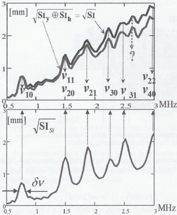
Fig. 9. Comparison of the models results. Explanation of the frequency peaks positions occurring in exact random model – \mathbf{SI}(\nu) , on the basis of the results of simplified (crystallographic) model \mathbf{SI}_{Si}(\nu)
