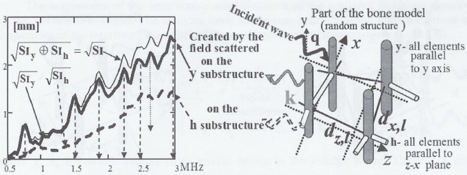
Fig. 5. Structural analysis of the scattered fields. Diagram of contributions of the selected substructures y, h in creation of the SI – I-st order BECS
