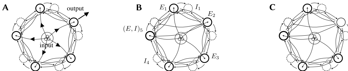
Figure 1. Five-node brain inspired neural network. A , a symmetric case. This basic case is then modified by: B , long-range connection E_2 \rightarrow (E, I)_5 , and C , removing access to the information source from neuron E_2 .
