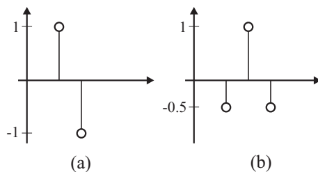
Figure 4: (a) Pulse inversion imaging. (b) Contrast pulse sequencing
