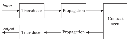
Figure 5: Block diagram for pulsing scheme evaluation system.
