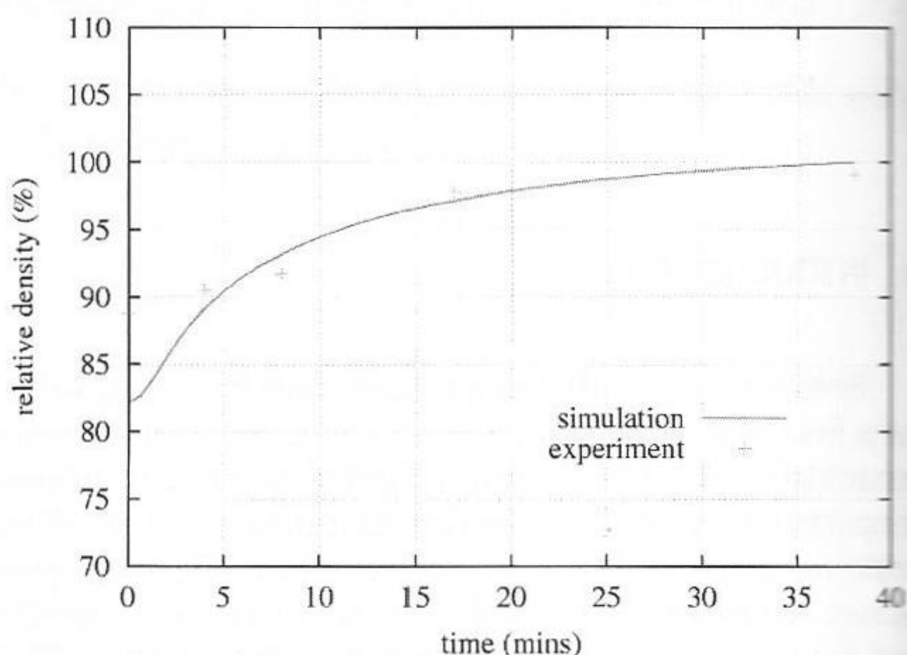
Fig. 5. Evolution of relative density during sintering process
