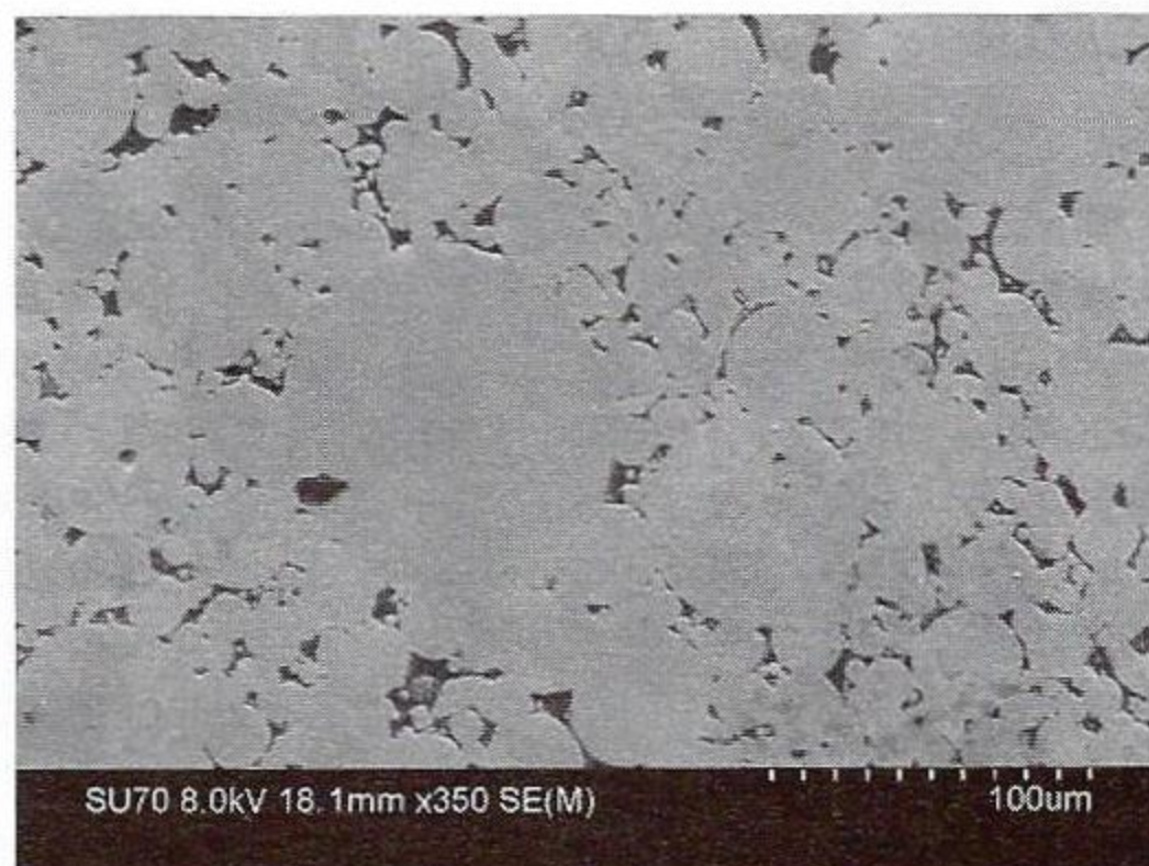
Fig. 2. Microstructure at an early stage of sintering of NiAl
