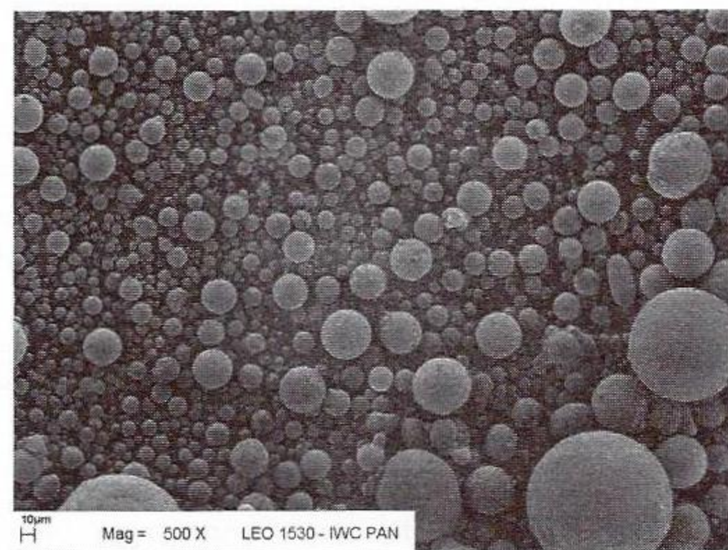
Fig. 1. Morphology of the NiAl powder
