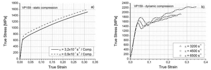
Fig. 1. Stress-strain curves of the X4CrMnN16-12 steel determined under static (a) and dynamic (b) loads
