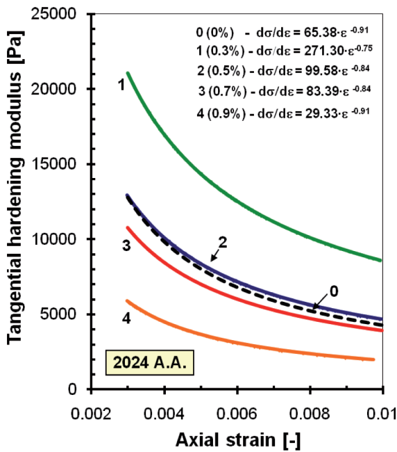
Fig. 6. Tangential hardening modulus calculated for the 2024 aluminium alloy on the basis of monotonic tension and cyclic torsion characteristic for strain amplitude within the range of \pm 0.3\% \div 0.9\%
