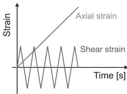
Fig. 1. Loading program
