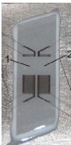
Fig. 3. Sensor delay line: 1 – channel with the sensor layer, 2 – reference channel.
