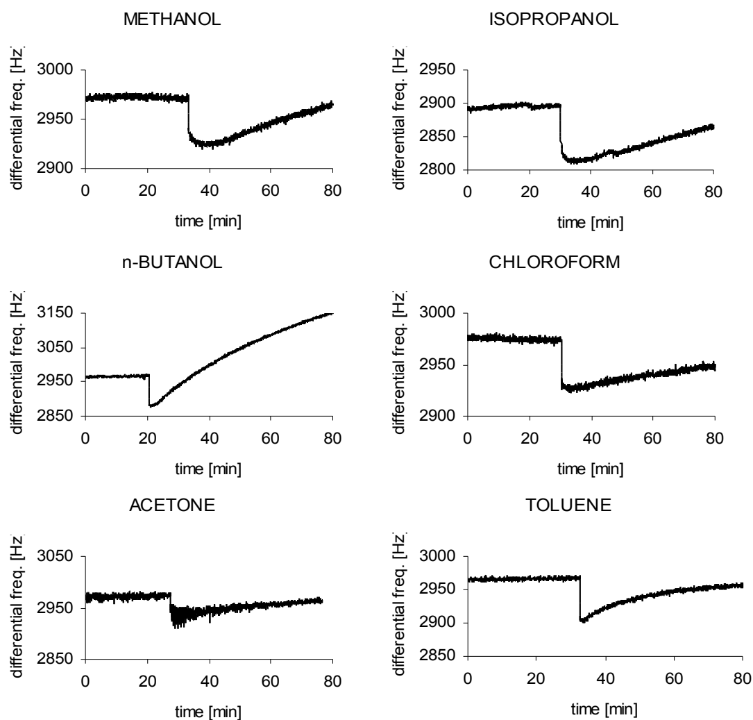
Fig. 5. Plot of the differential frequency vs. time for the sensor delay line with the layer of DA+CA in the air with 3.5% (mass) vapour of some VOC.
